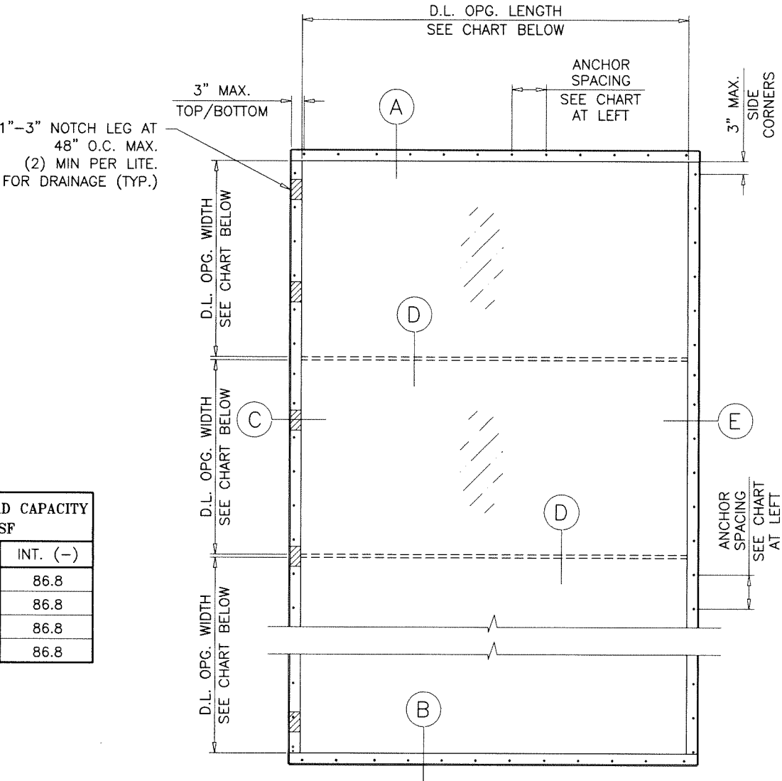
TYPICAL ELEVATION
